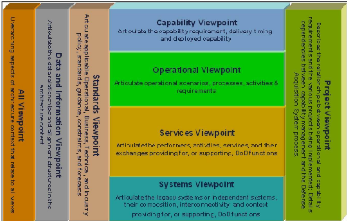
DoDAF Viewpoints
